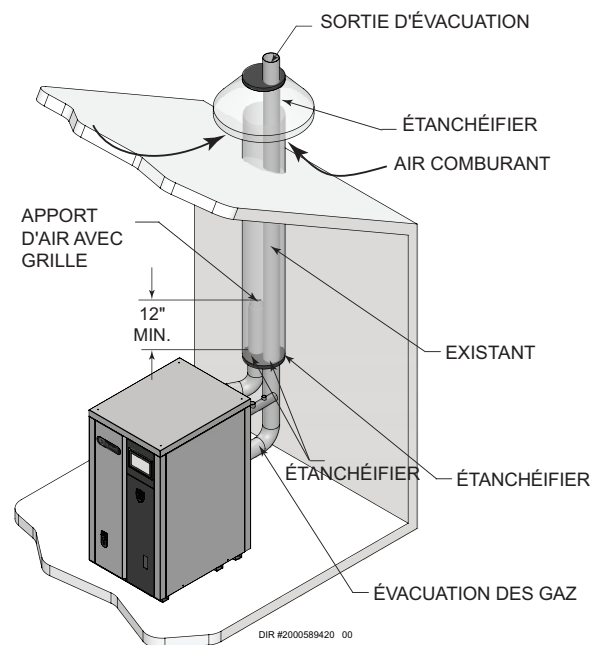
Figure 5-8 Ventilation concentrique, exemple 1
